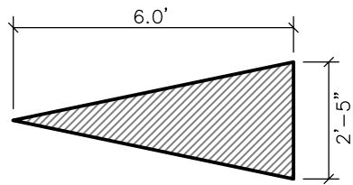
TYPICAL PAVEMENT MARKINGS NTS
