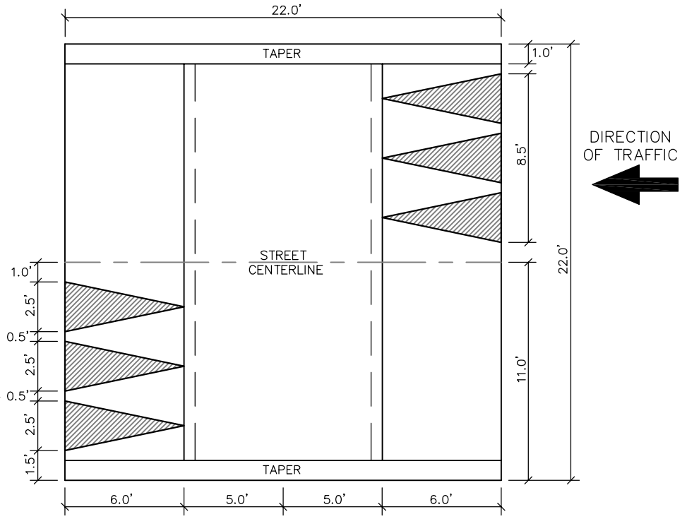
TYPICAL PAVEMENT MARKINGS NTS
