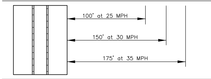
ROAD SPEED AND SIGN PLACEMENT NTS
