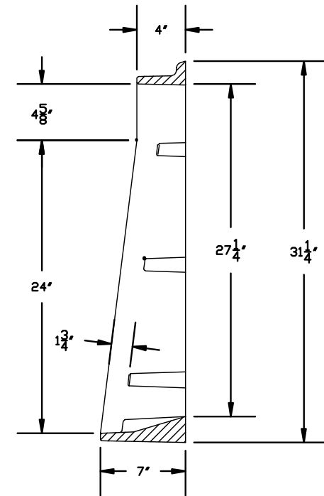
FRAME SECTION
