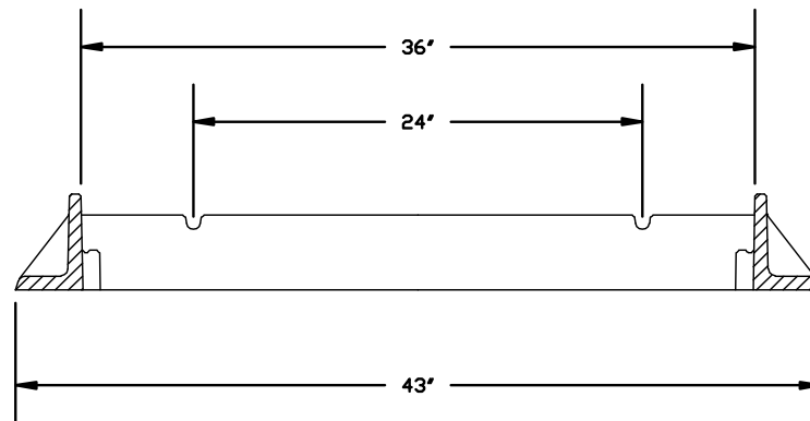
FRAME SECTION
