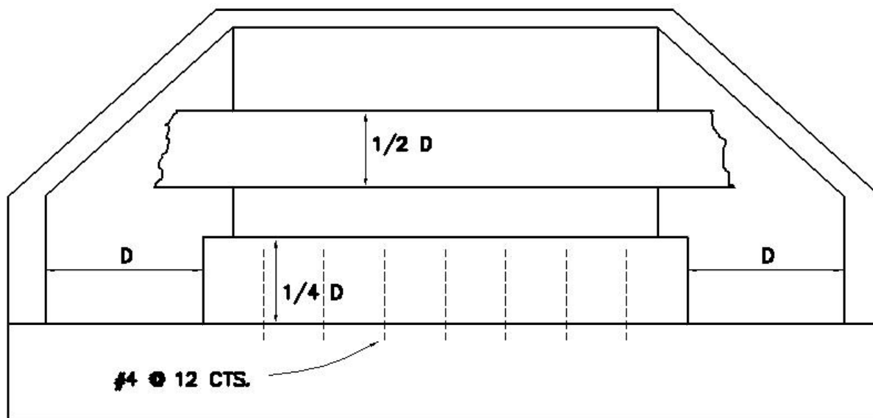
FRONT ELEV.
