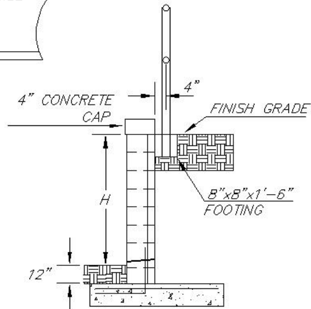
INSTALLATION FOR WALLS LESS THAN 12" THICKNESS (NTS)
