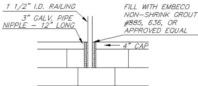
INSTALLATION FOR WALL 12" AND LARGER IN THICKNESS
