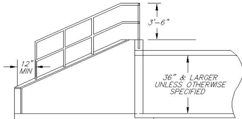
RAILING FOR HEADWALL/WINGWALL INSTALLATIONS (NTS)
