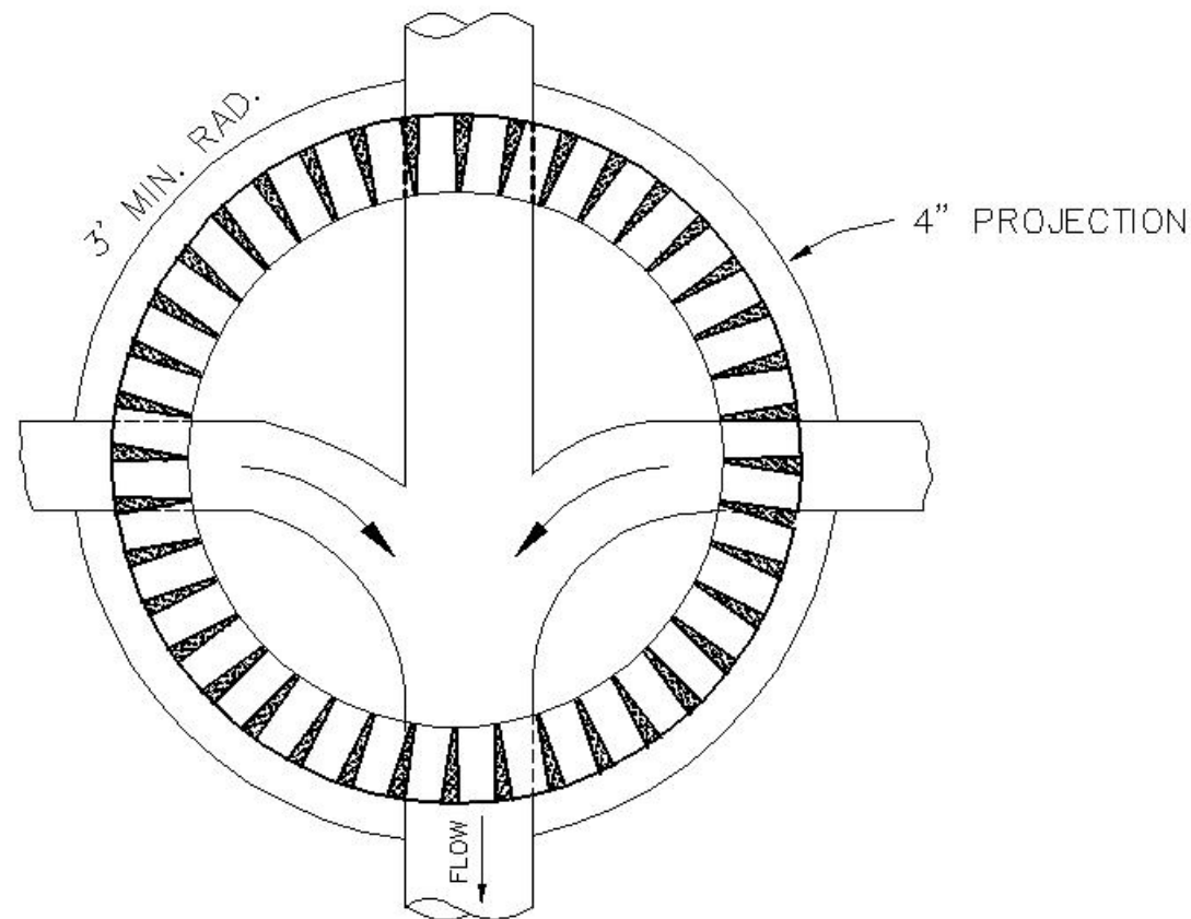
PLAN SHOWING LATERALS SIDE OF CHANNEL TO BE SLOPED 1"/FT
