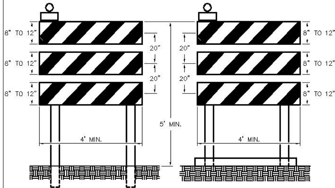
TYPE III BARRICADE (FIXED)
